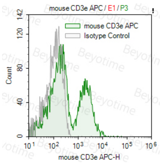
图1. 碧云天APC anti-mouse CD3e (AC0939)检测效果图。C57BL/6J splenocytes stained with APC anti-mouse CD3 (clone BY145-2C11) (colored histogram) or APC Hamster IgG (gray histogram).
